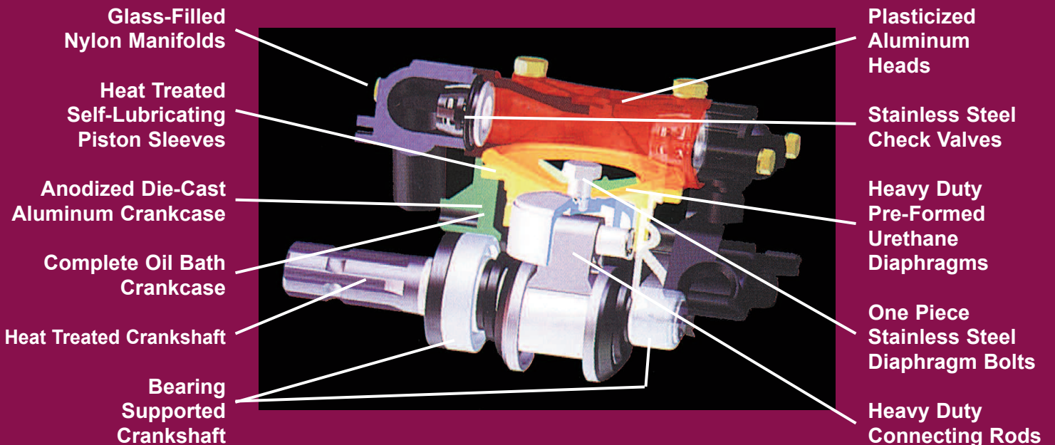
UDOR RO Series Diaphragm Pump
